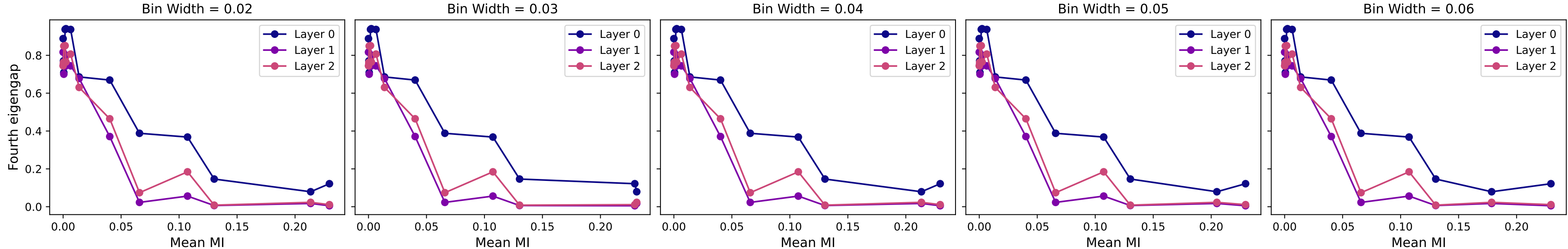
Mutual Information vs Fourth Eigengaps (13 datasets)
